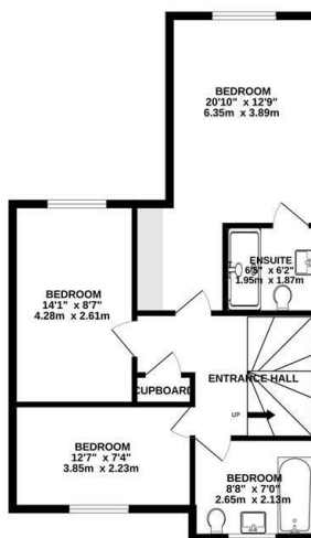
1ST FLOOR 610 sq.ft. (56.6 sq.m.) approx.
